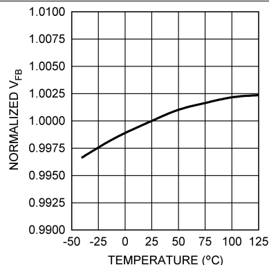
Figure 8. Normalized Feedback Voltage vs Temperature
