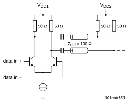
Fig 6. AC coupling
