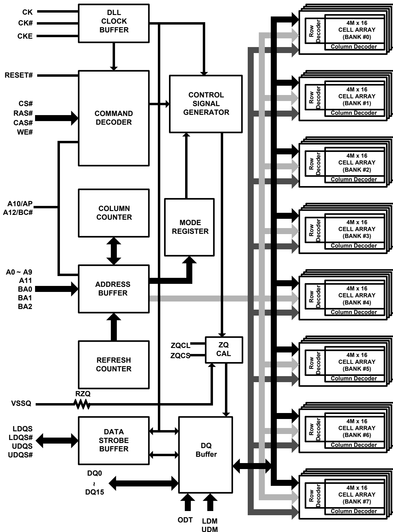
Figure 2. Block Diagram
