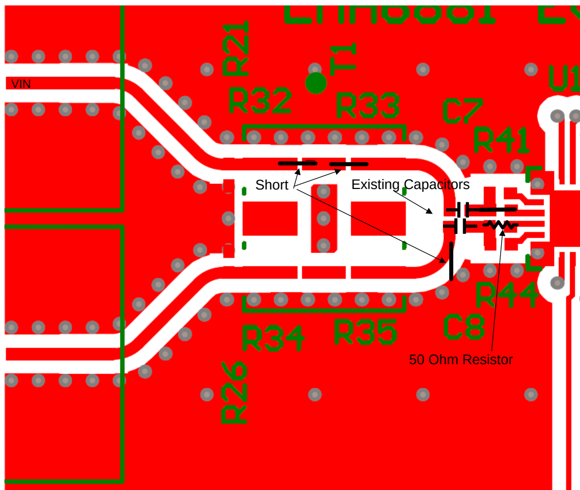
Figure 4. Input Configuration for Single Ended Signal. R44 should be 50Ω to ground. R32, 33 are 0Ω shorts. R34 and R35 are not needed.
