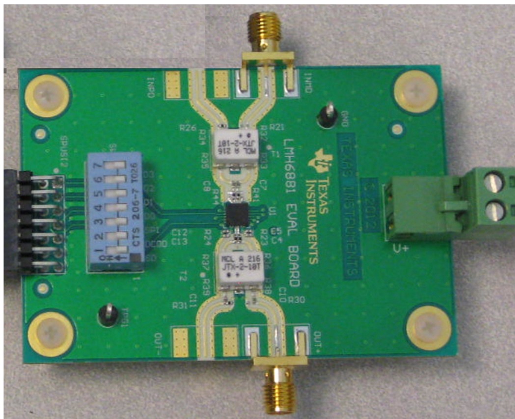
Figure 1. LMH6881 Evaluation Board
