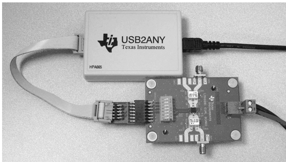
Figure 5. Evaluation Board
