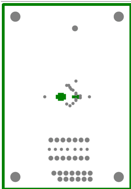
Figure 11. Layer 2, Ground
