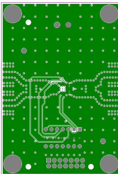
Figure 13. Layer 6, 5V Power
