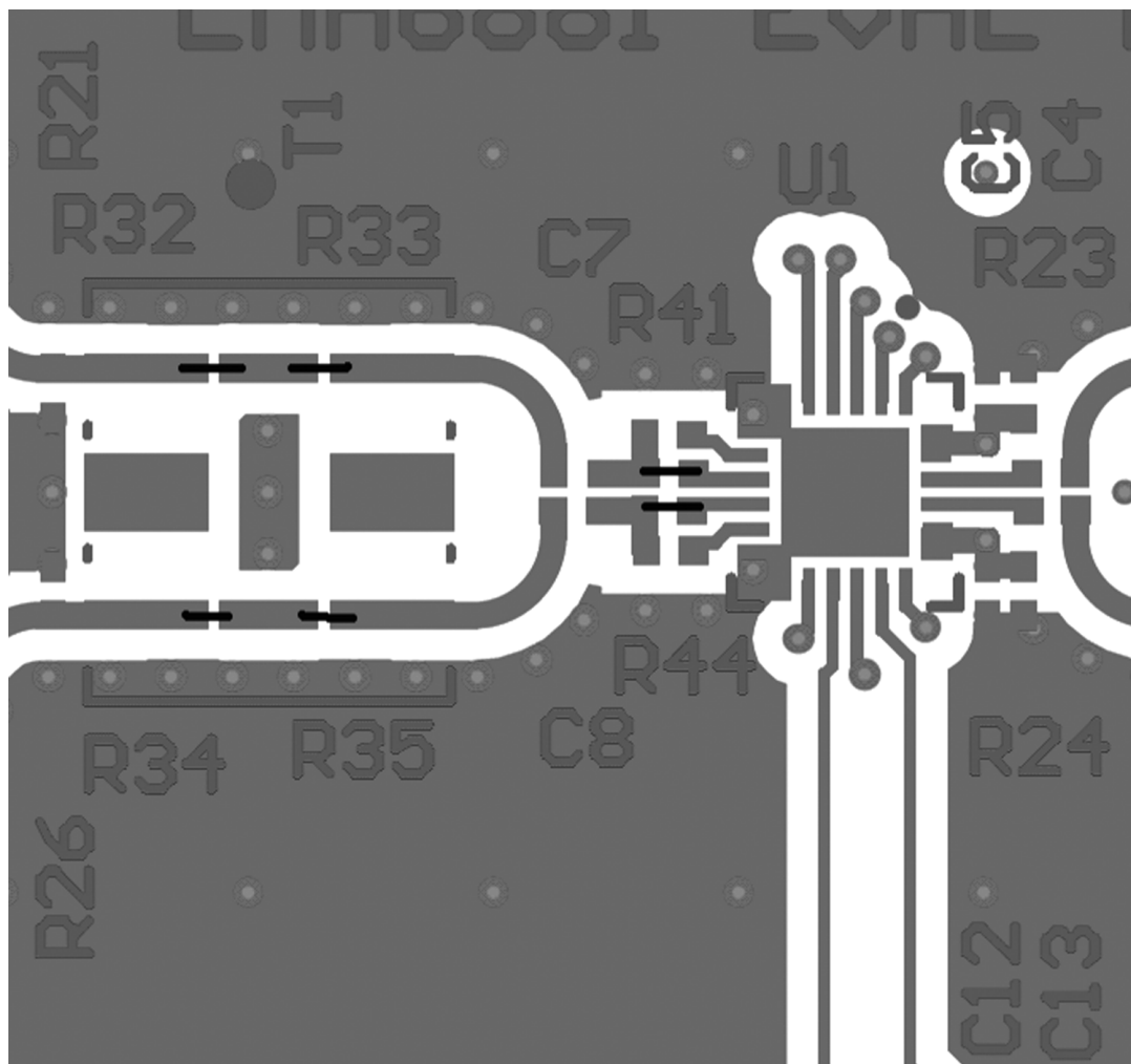
Figure 3. Input Configuration for Differential Signals. Black lines indicate shorts or 0Ω resistors.
