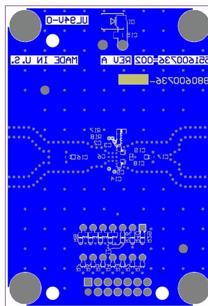
Figure 10. Bottom Layer
