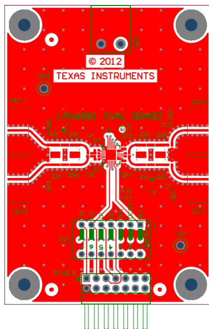
Figure 9. Top Layer
