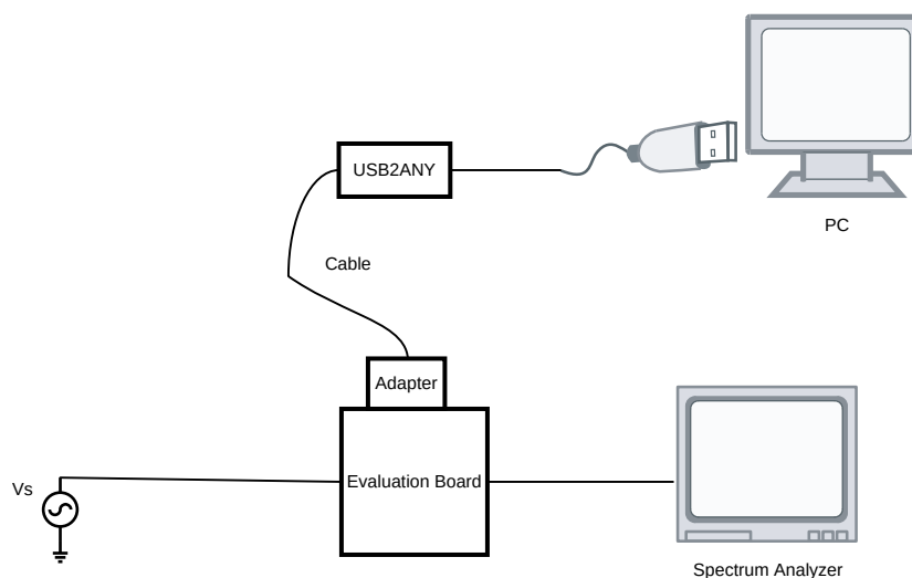
Figure 6. Typical Bench Setup
