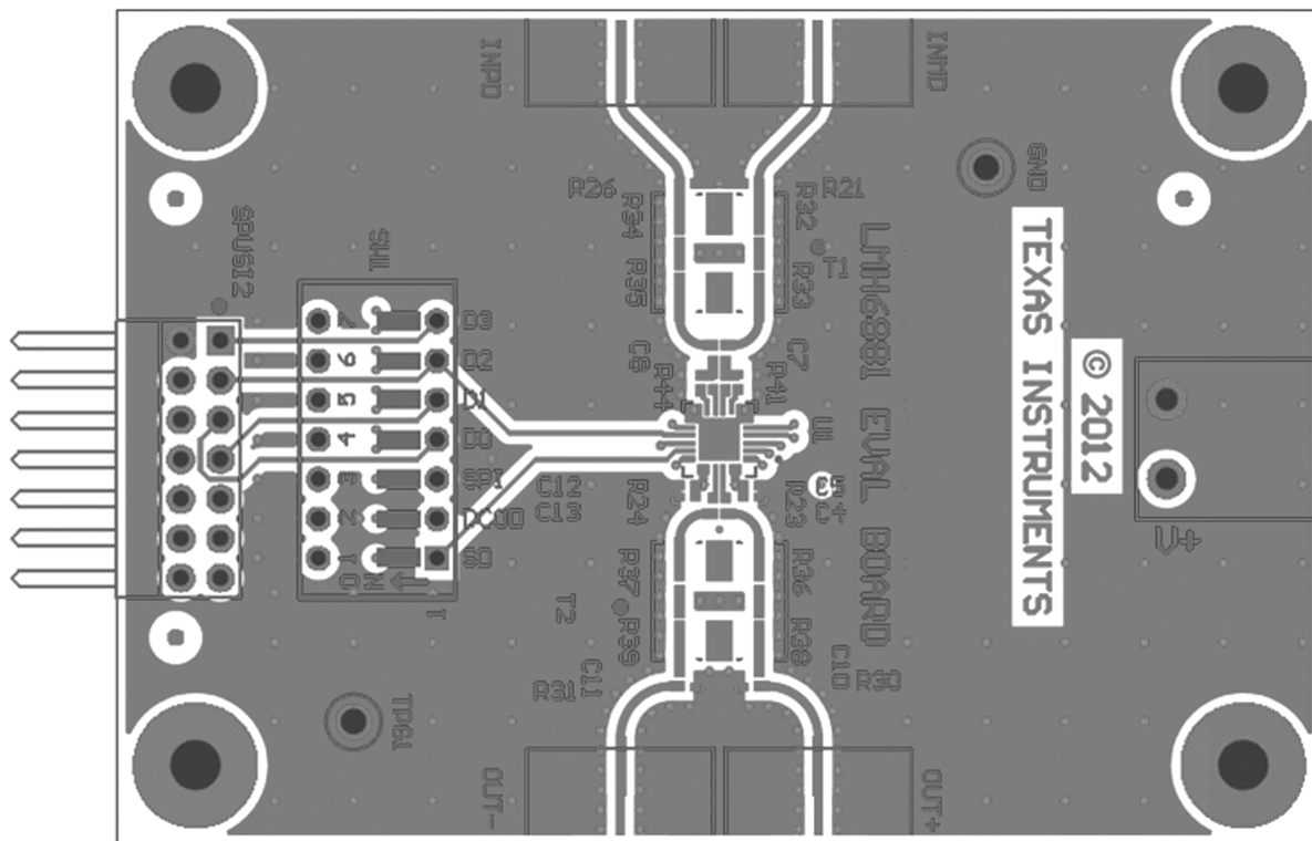
Figure 2. Top Layer Metal
