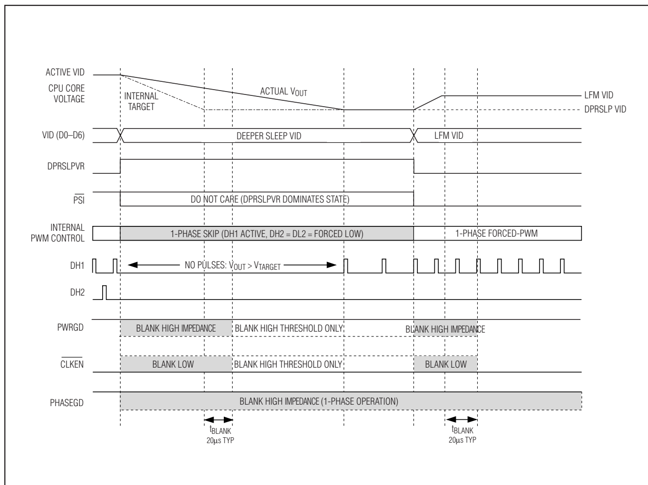
Figure 5. Standard C4 Transition
