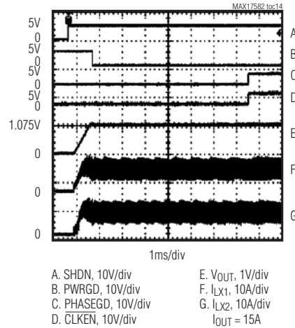
SOFT-START WAVEFORM (UP TO PWRGD)
