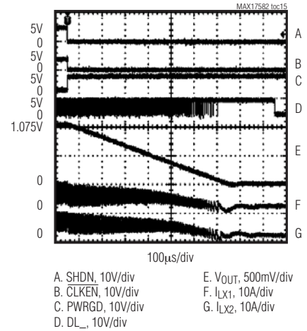
SHUTDOWN WAVEFORM
