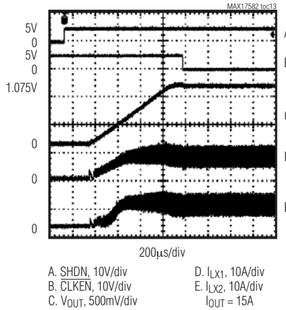
SOFT-START WAVEFORM (UP TO CLKEN)
