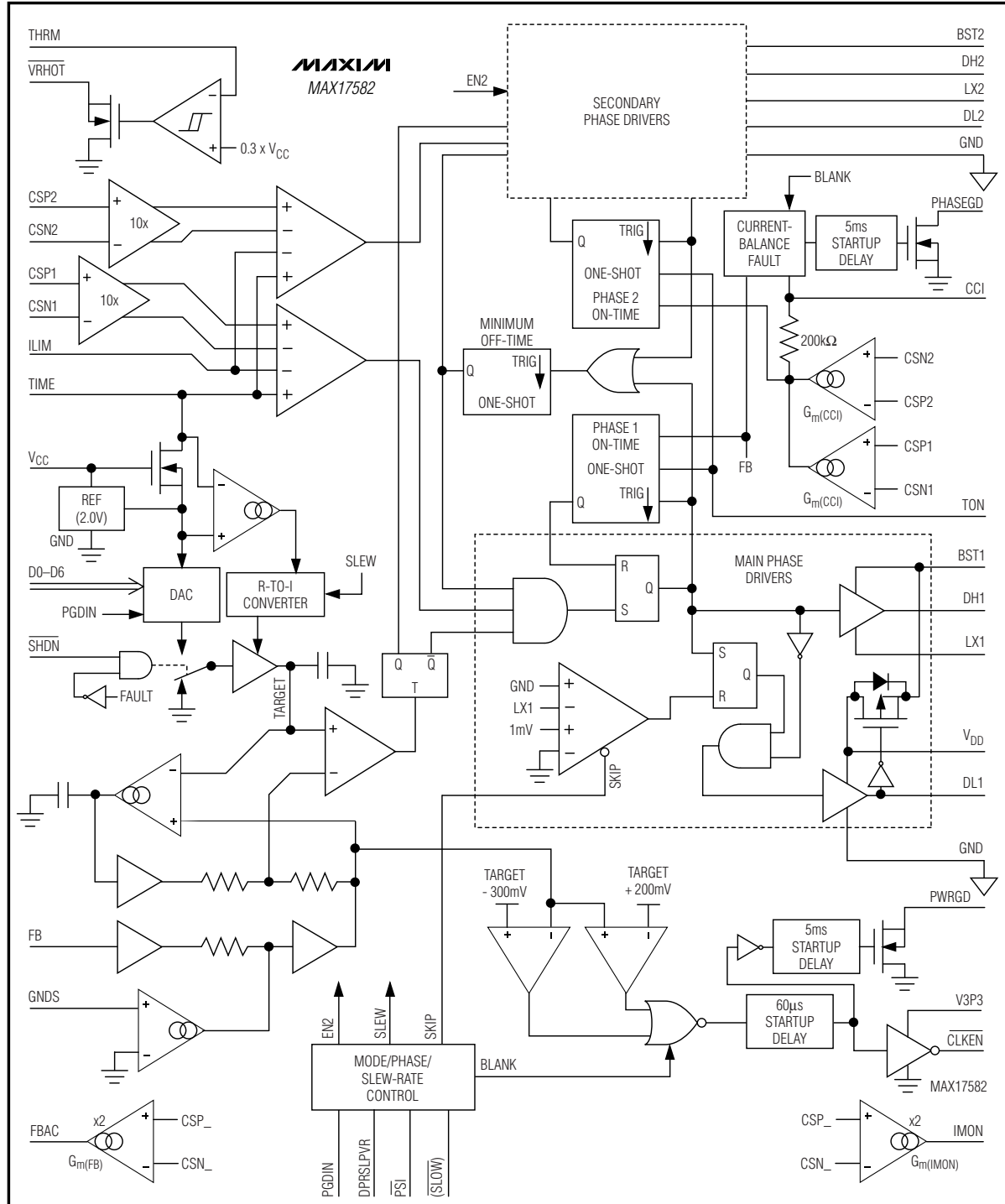
Figure 2. Functional Diagram
