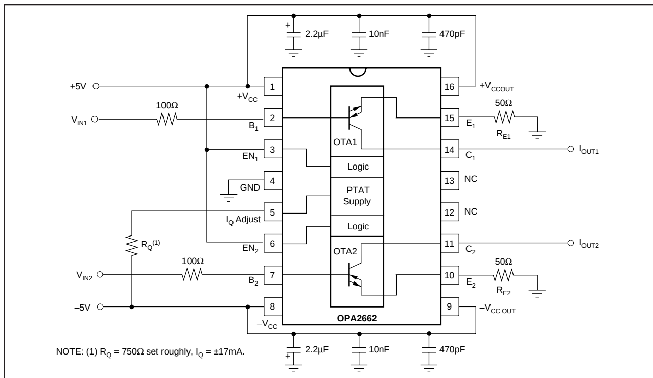
FIGURE 6. Basic Connections.
