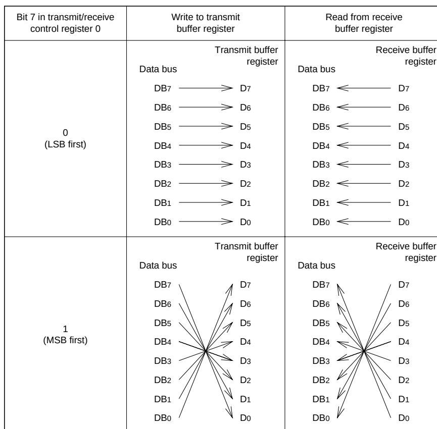
Fig. 62 Connection relation between transmit buffer register, receive buffer register, and data bus
