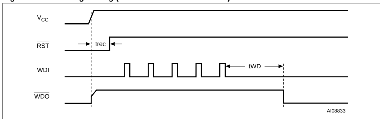
Figure 31. Watchdog Timing (STM706T/S/R and STM706P)
