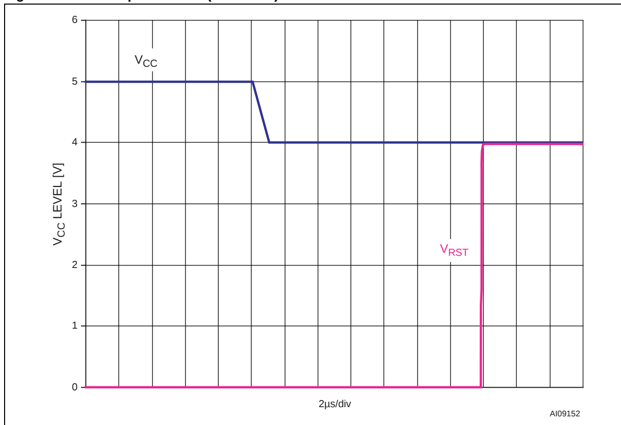
Figure 23. RST Response Time (Assertion)
