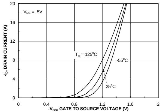
Figure 16. Transfer Characteristics.
