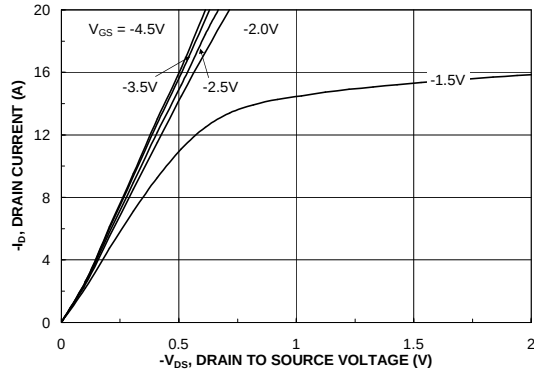
Figure 12. On-Region Characteristics.
