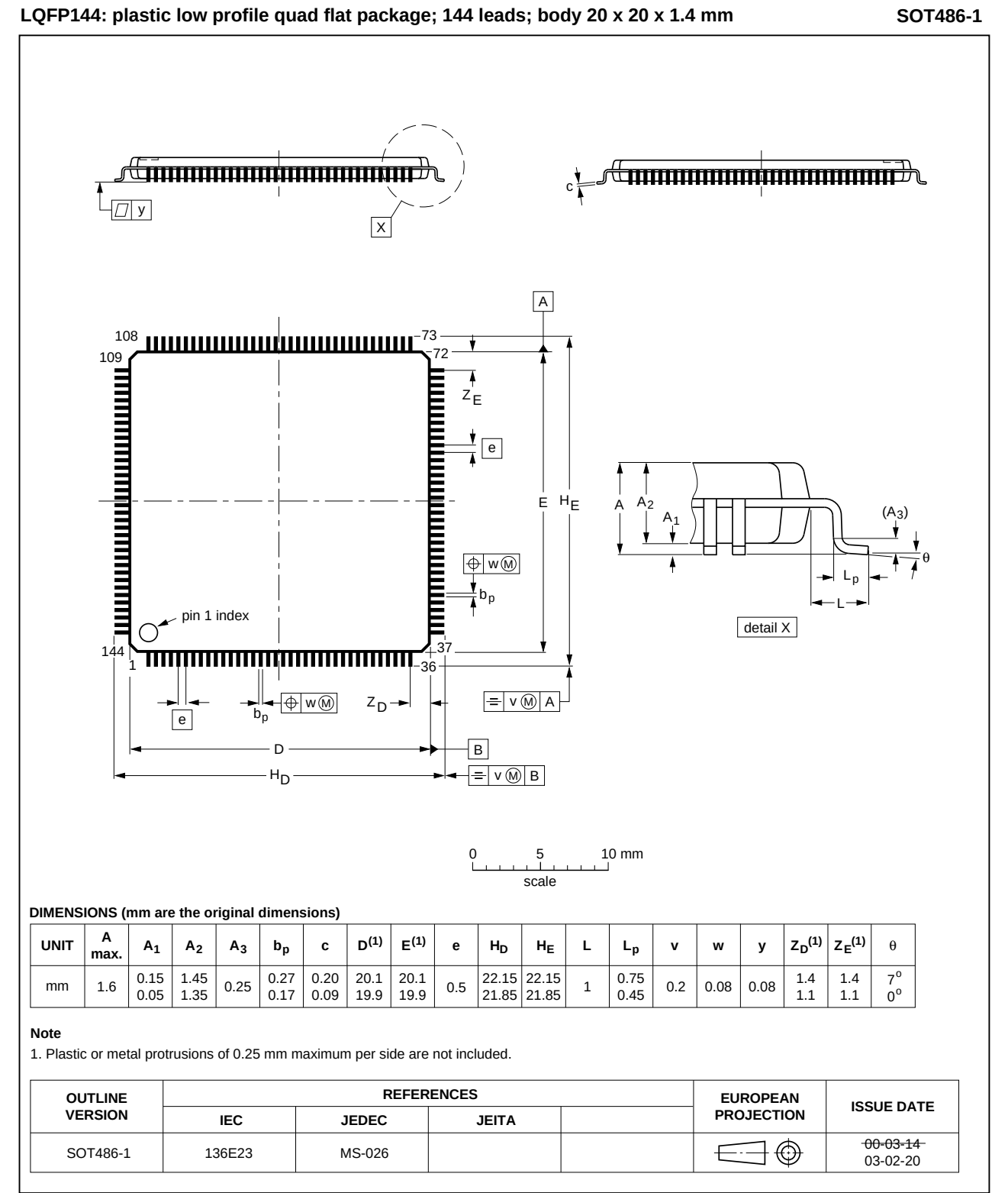
Fig 26. Package outline SOT486-1 (LQFP144)
