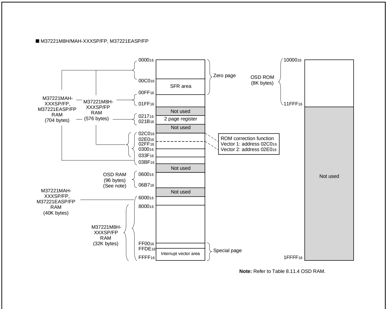
Fig. 8.2.2 Memory Map (M37221M8H/MAH-XXXSP/FP, M37221EASP/FP)
