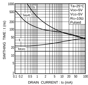
Fig.19 Switching characteristics
