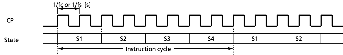
Figure 2-19. Instruction Cycle
