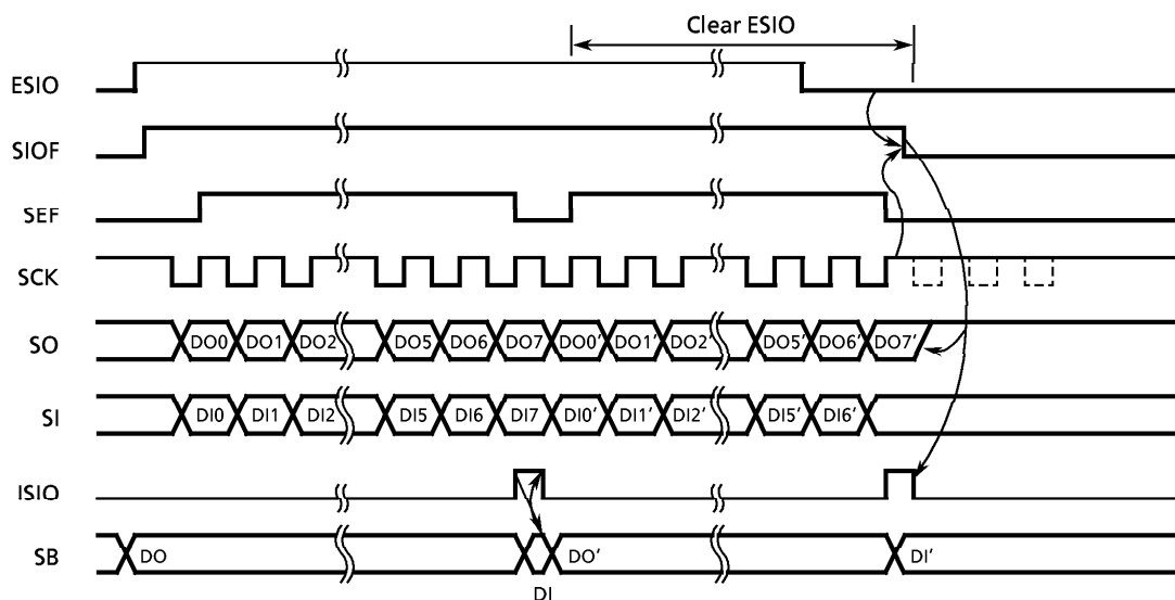
Figure3-35. 8-bit Transmit/Receive Mode
