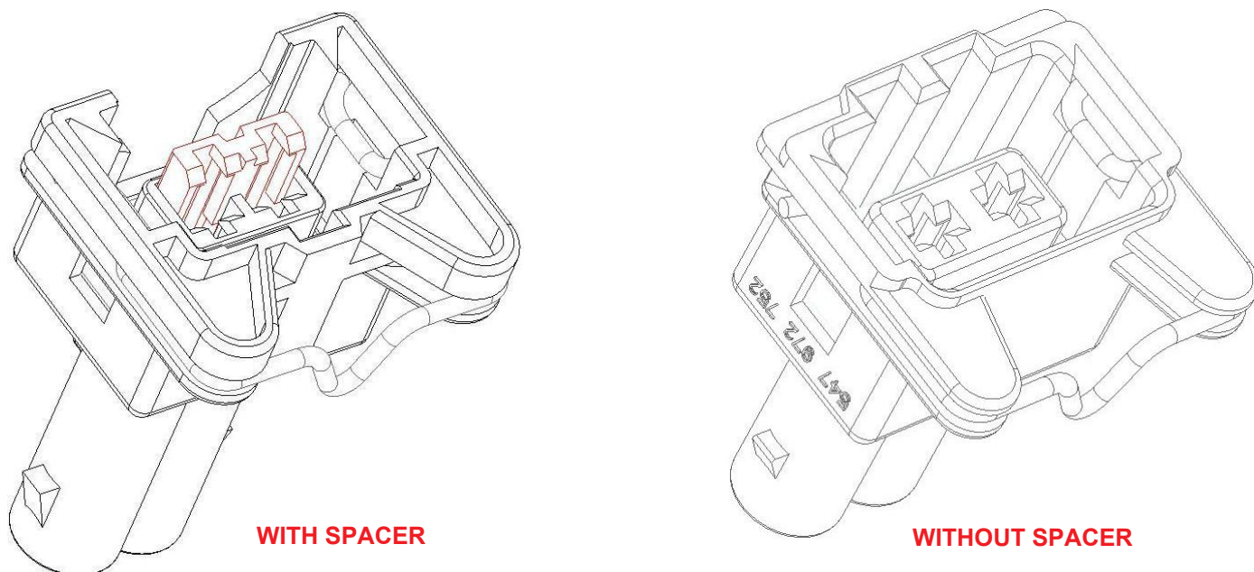
HOUSING ASS'Y 2 POS. JUNIOR POWER TIMER REC.
