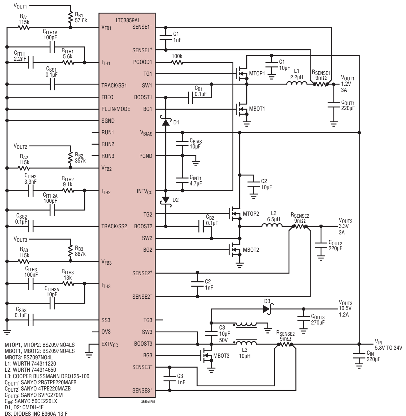
Figure 15. High Efficiency 1.2V/3V Step-Down Converter with 10.5V SEPIC Converter
