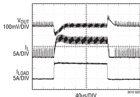
Transient Response (Discontinuous Mode)
