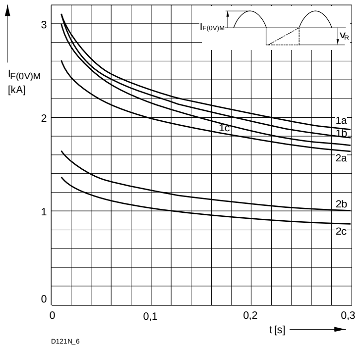
Bild / Fig. 4 Grenzstrom / Maximum overload forward current I_{F(0V)M} = f(t) 1 - I_{FAV(vor)} = 0\text{ A} ; t_{vj} = t_c = 25\text{ °C} 2 - I_{FAV(vor)} = 120\text{ A} ; t_c = 113\text{ °C} ; t_{vj} = 180\text{ °C} a - v_R \leq 50\text{ V} b - v_R = 0,5\text{ V RRM} c - v_R = 0,8\text{ V RRM}
