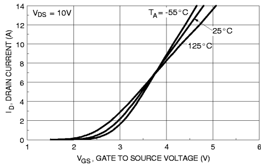
Figure 5. Transfer Characteristics.
