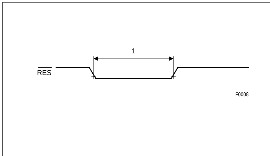
Figure 81 Reset Timing
