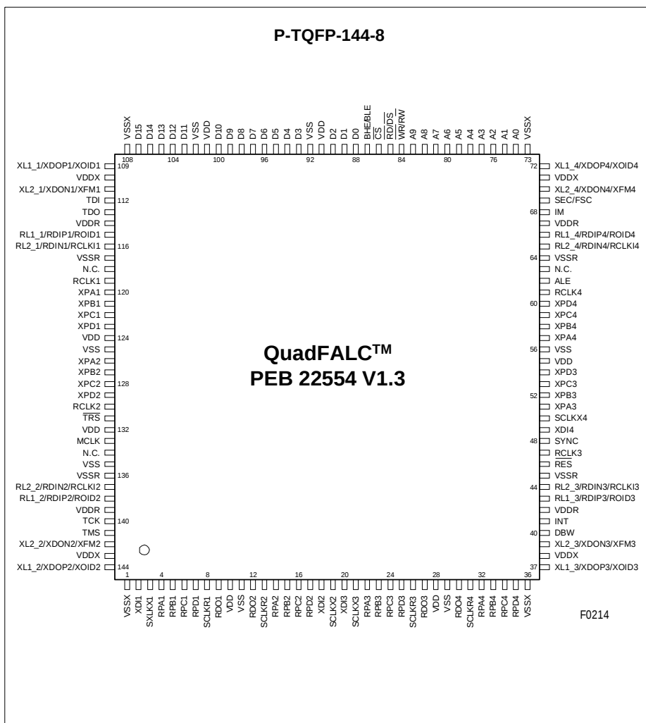
Figure 4 Pin Configuration
