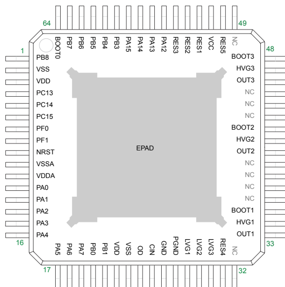
Figure 2. STSPIN32F060x pin connection (TQFP top view)
