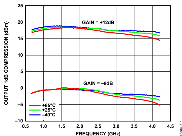
Figure 7. Output 1dB Compression vs. Frequency for Various Temperatures and Gains, V_{POS} = 5\text{ V}
