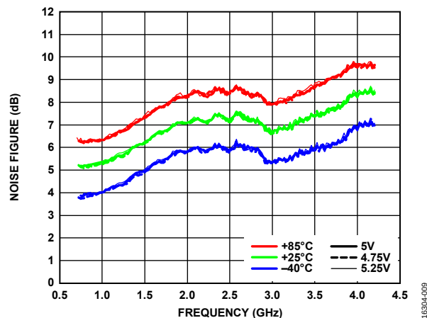
Figure 9. Noise Figure vs. Frequency for Various Temperatures and V_{POS} at Maximum Gain = 12 dB
