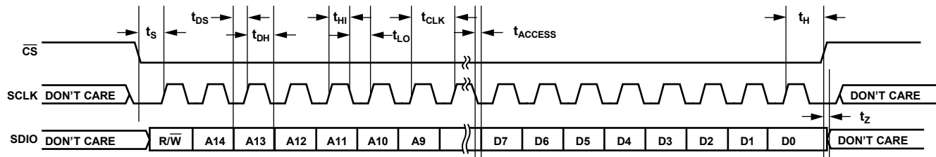
Figure 2. SPI Timing
