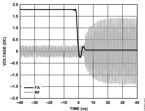
Figure 21. Fast Attack Response, Off at 16 dB
