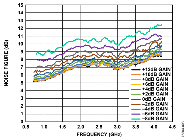
Figure 8. Noise Figure vs. Frequency for Various Gain Steps at V_{POS} = 5\text{ V}
