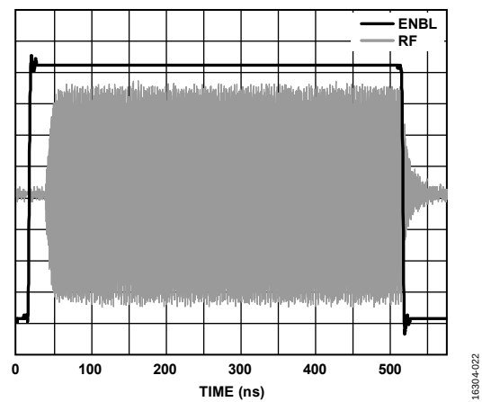
Figure 22. Enable/Disable Time Domain Response
