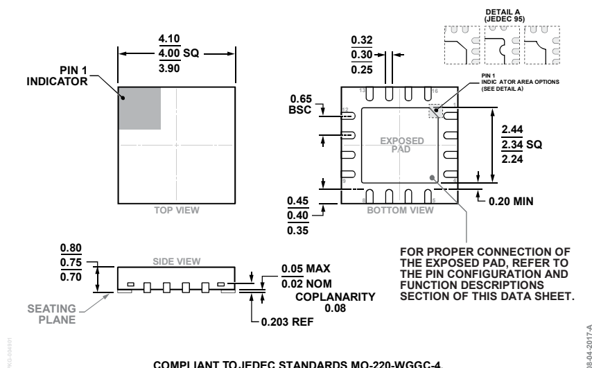
COMPLIANT TO JEDEC STANDARDS MO-220-WGGC-4. Figure 26. 16-Lead Lead Frame Chip Scale Package [LFCSP] 4 mm × 4 mm Body and 0.75 mm Package Height (CP-16-39) Dimensions shown in millimeters
