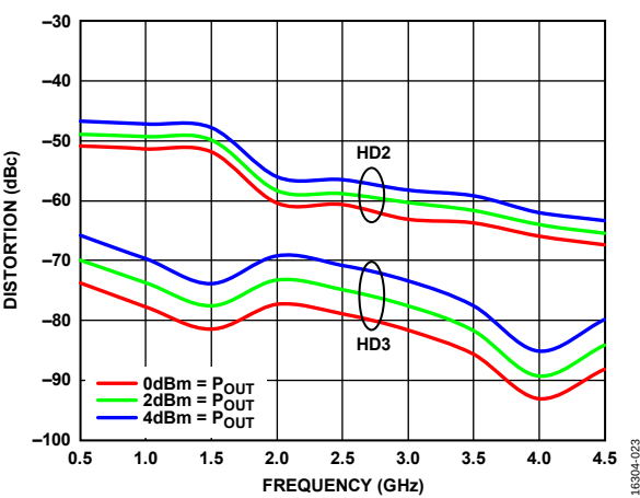
Figure 23. Distortion (HD2 and HD3) vs. Frequency for Various Output Powers ( P_{OUT} )
