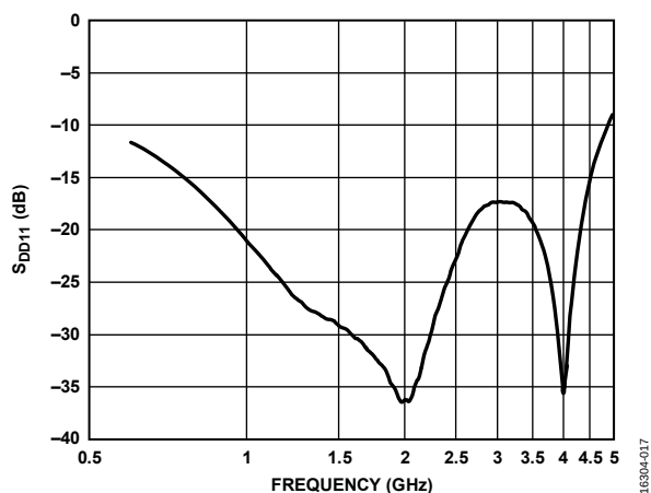
Figure 17. Input Reflection Coefficient ( S_{D11} ) vs. Frequency, Gain = 12 dB
