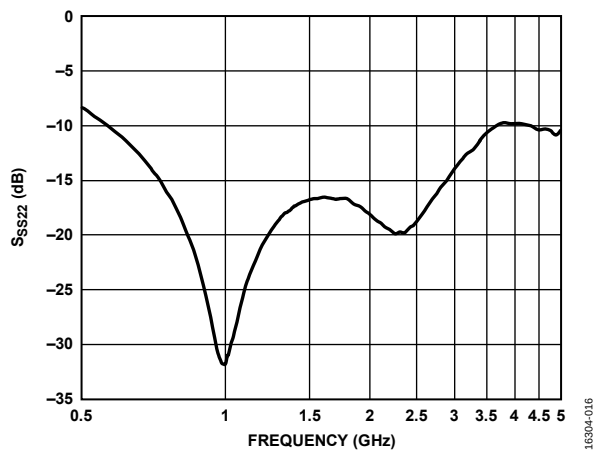
Figure 16. Output Reflection Coefficient ( S_{S22} ) vs. Frequency, Gain = 12 dB
