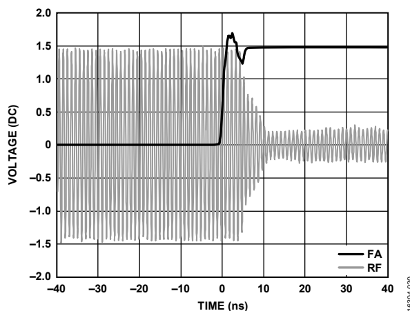
Figure 20. Fast Attack Response, On at 16 dB
