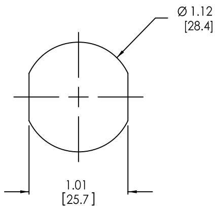
PANEL CUT-OUT
