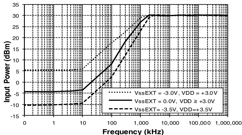
Figure 4. Maximum Operating Power vs. Frequency ( T_{\text{ambient}} = 25^{\circ}\text{C} )
