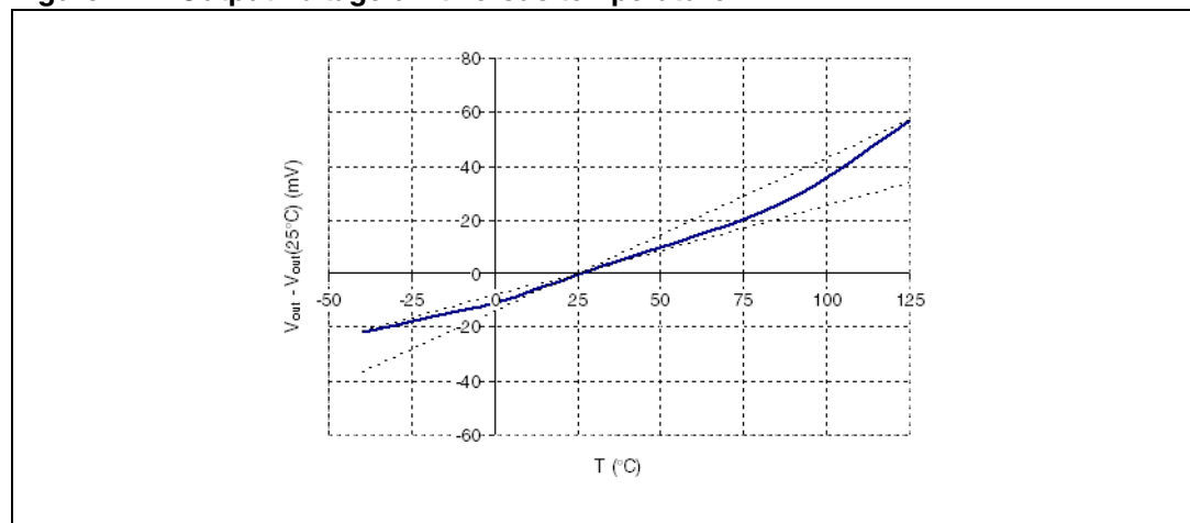
Figure 21. Output voltage drift versus temperature
