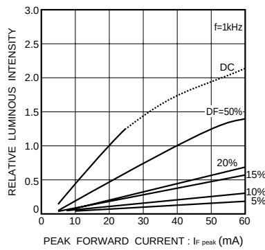
Fig.24 Luminous intensity vs. peak forward current
