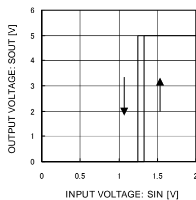
Fig.9 SIN Detect Voltage
