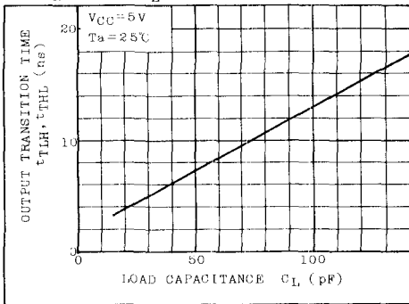
t_{TLH}, t_{THL} - C_L CHARACTERISTICS (TYP.)
