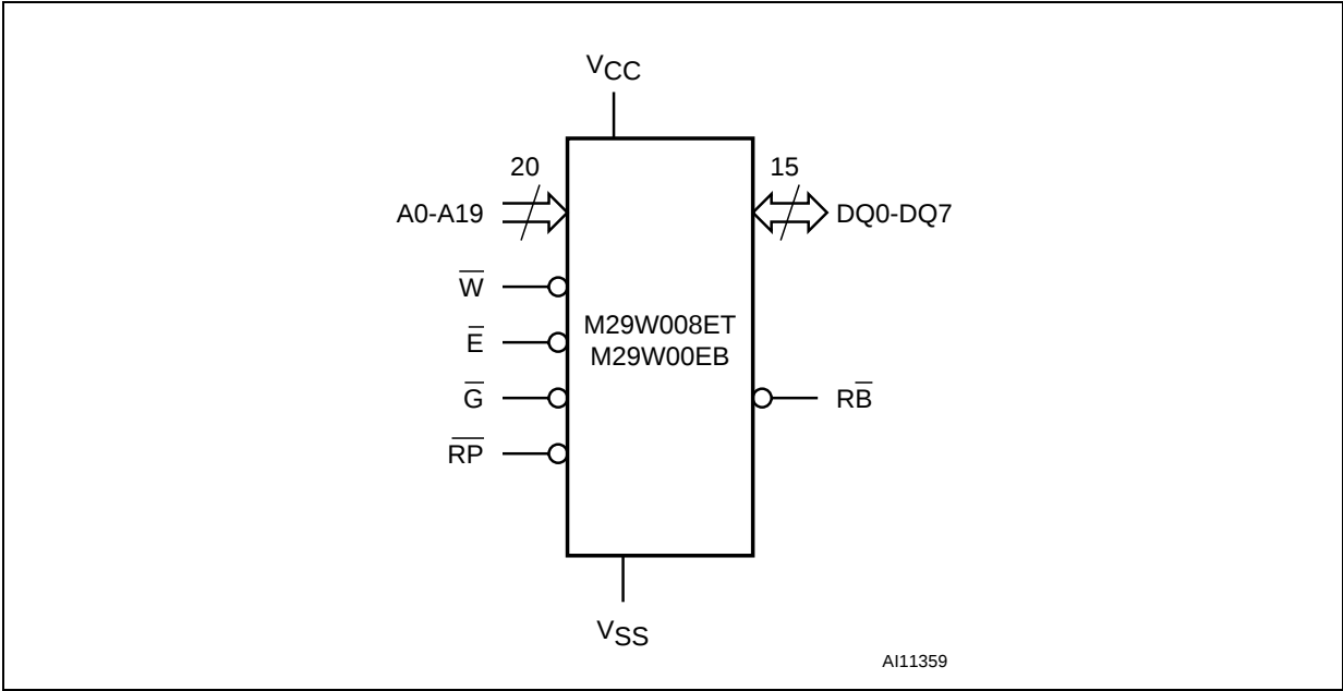
Figure 2. Logic diagram
