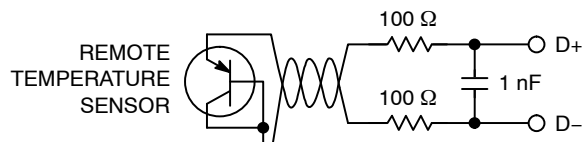
Figure 22. Filter Between Remote Sensor and ADT7482
