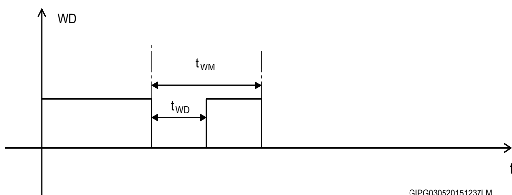
Figure 11. Watchdog reset
