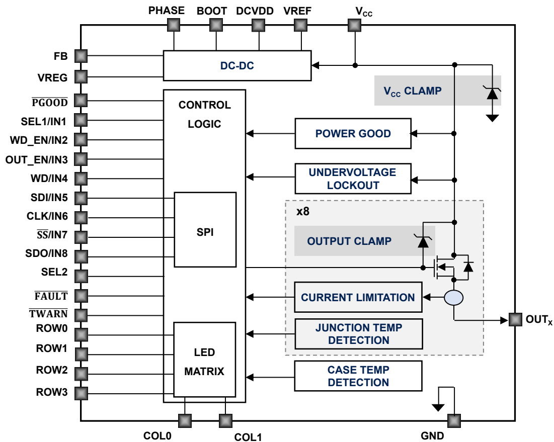
Figure 1. Block diagram
