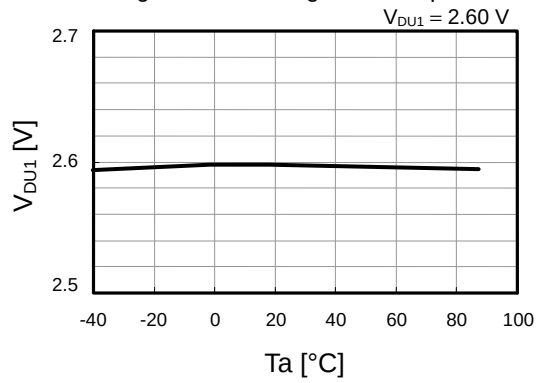
Overcurrent1 detection voltage vs. temperature
