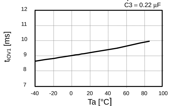
Overcurrent1 detection time vs. temperature
