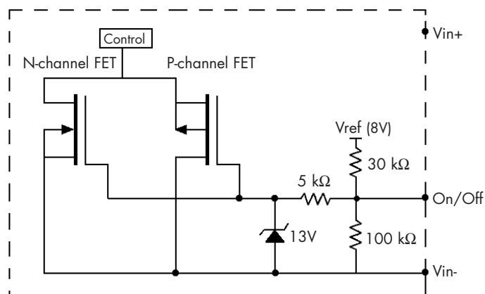
Figure B: Internal ON/OFF pin circuitry
