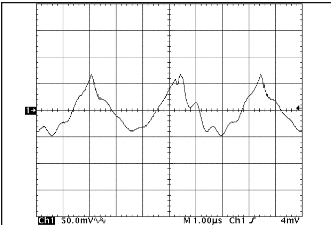
Figure 15: Output voltage ripple at nominal input voltage and rated load current (50 mV/div). Load capacitance: 1\mu F ceramic capacitor and 15\mu F tantalum capacitor. Bandwidth: 20 MHz. See Figure 12.
