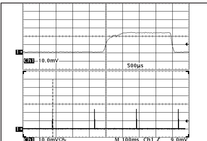
Figure 17: Load current (50A/div) as a function of time when the converter attempts to turn on into a 1\text{ m}\Omega short circuit. Top trace (500μs/div) is an expansion of the on-time portion of the bottom trace.
