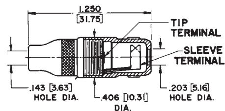
TINI-EXTENSION JACK
