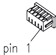
Molex 51021-0500 "CONN 1"
