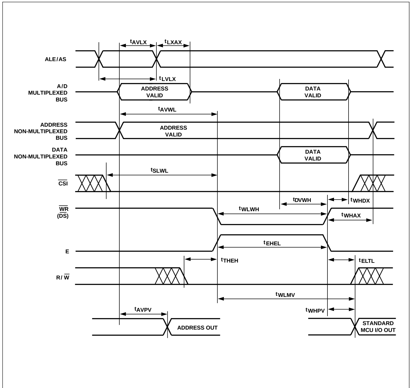
Figure 28. Write Timing
