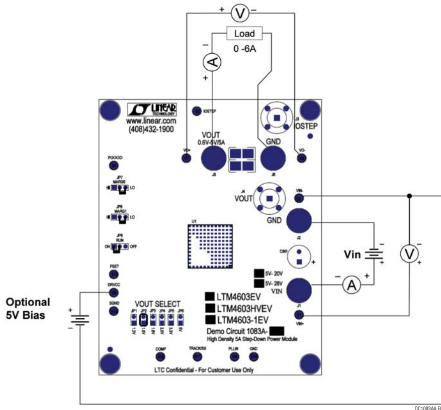
Figure 1. Test Setup of DC1083A-A (DRV CC Bias Supply is Optional)
