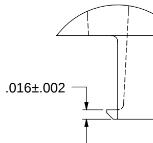
DETAIL A SCALE=6X
