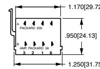
MARKING DETAIL FRONT VIEW VCH CONNECTOR HOUSING
