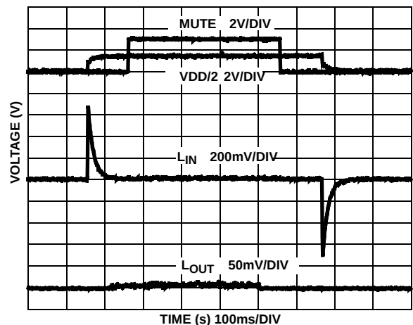
FIGURE 29. 1k\Omega AC-COUPLED CLICK AND POP REDUCTION
