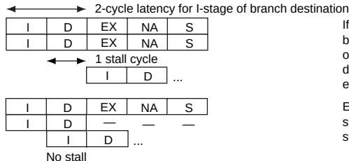
Figure 8.3 Examples of Pipelined Execution
