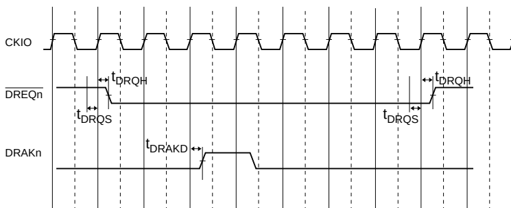
Figure 23.64(a) \overline{DREQ} /DRAK Timing
