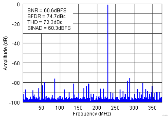
Figure 7-4. FFT for 230-MHz Input Signal (Auto On)
