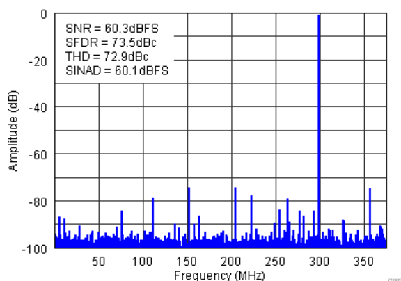
Figure 7-6. FFT for 450-MHz Input Signal (Auto On)
