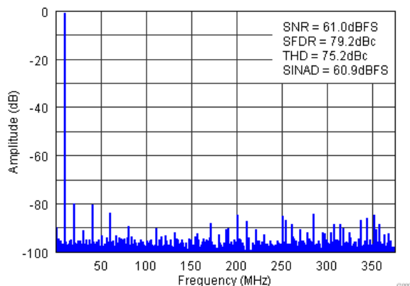
Figure 7-2. FFT for 10-MHz Input Signal (Auto On)
