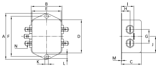
Connection style -06, 1 to 12 A types
