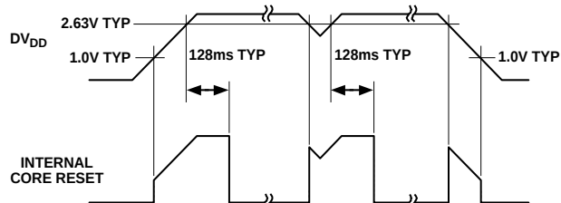
Figure 66. 3 V Part POR operation
