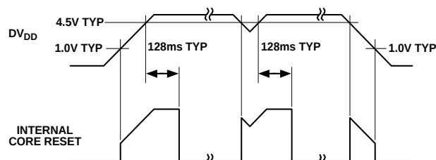
Figure 67. 5 V Part POR Operation
