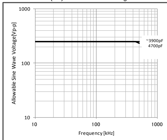
C0G(5C) Char. Rated Voltage : DC250V
