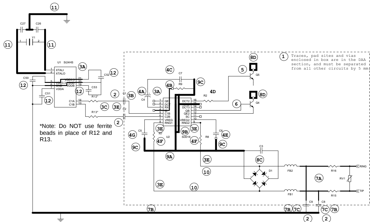
Note: Encircled references are described in the numbered paragraphs in Appendix A. This is not a complete schematic. Only critical component placement and nets are drawn.
