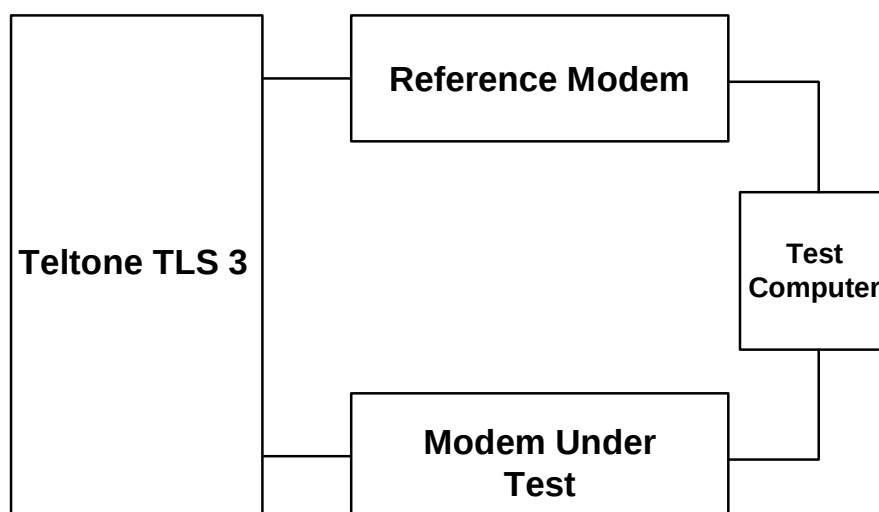
Figure 48. Bell 103–V.34 Modem Functional Test Connection
