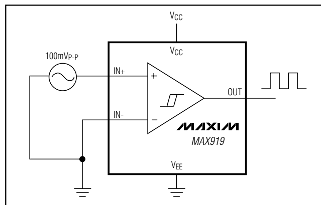
Figure 5. Zero-Crossing Detector
