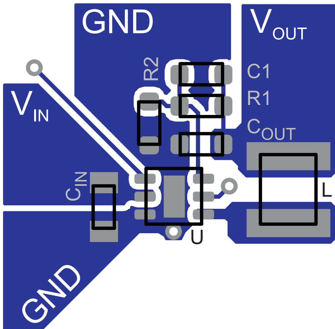
Figure 40. Suggested Layout for Adjustable Output Voltage Version
