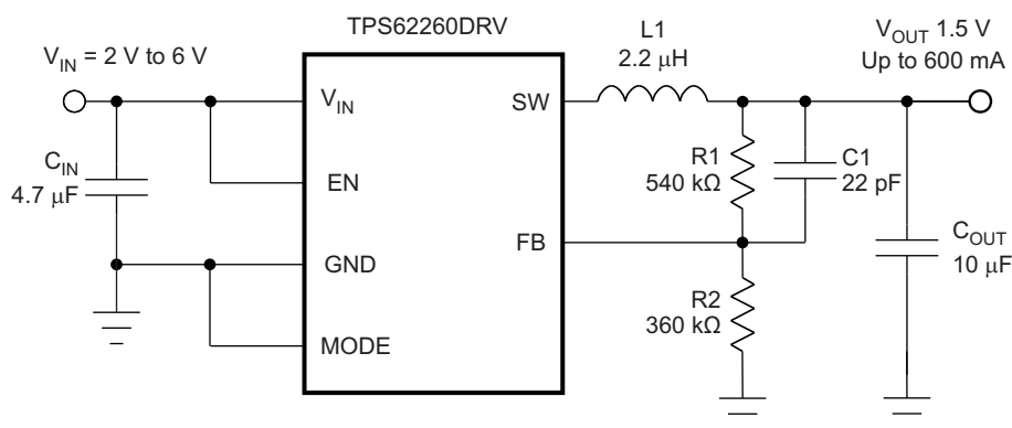
Figure 37. TPS62260 adjustable 1.5-V Output
