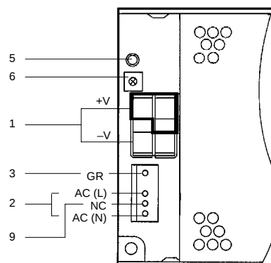
Connector Model
