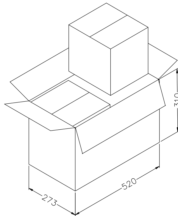
OUTER CARTON BOX 2 INNER CARTON BOXES PER CARTON QTY: 2 X 2000 = 4000PCS DIMENSION IN MM
