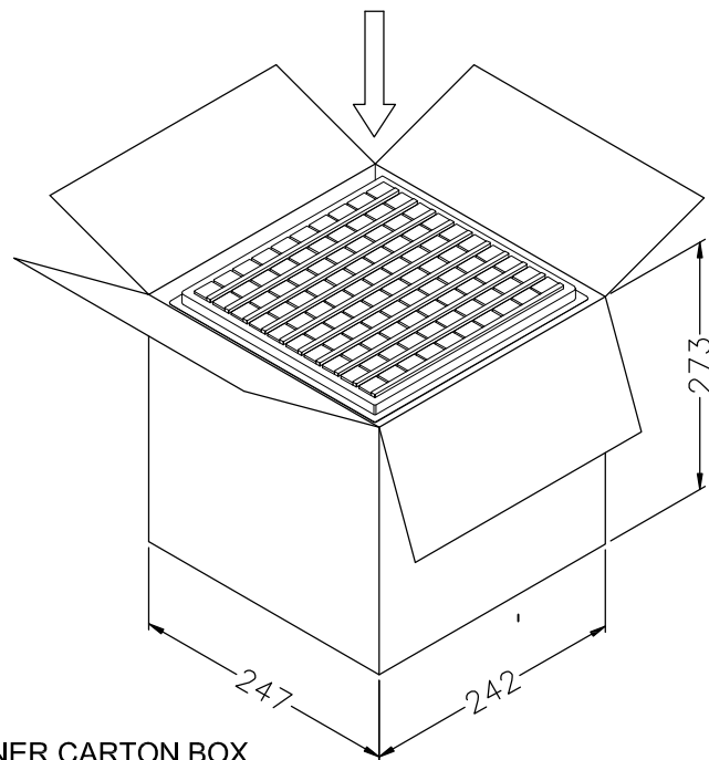
INNER CARTON BOX 20 PVC TRAYS PER CARTON QTY: 20 X 100 = 2000PCS DIMENSION IN MM
