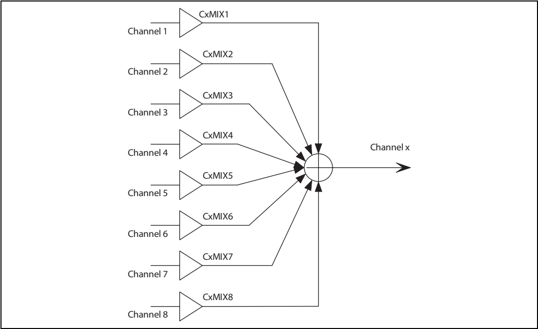
Figure 8. Channel mixer
