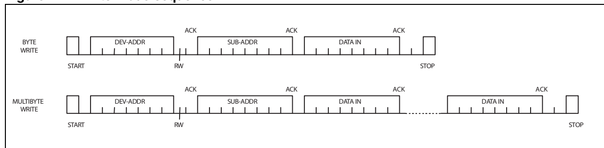
Figure 4. Write mode sequence
